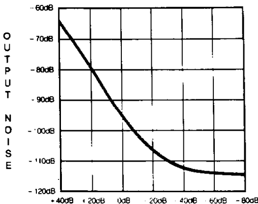
CURRENT GAIN/ATTENUATION NOISE BANDWIDTH (20Hz-20kHz) (Referred to 600\mu A_{pp} Input Signal 12dB of Headroom)
