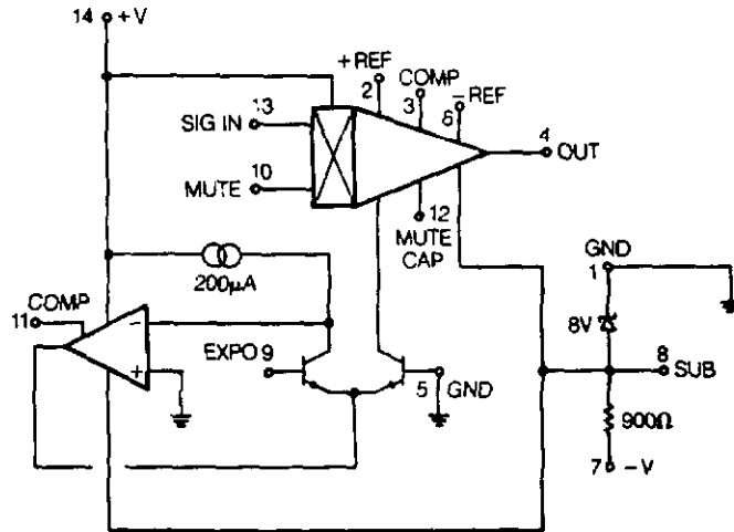
BLOCK DIAGRAM
