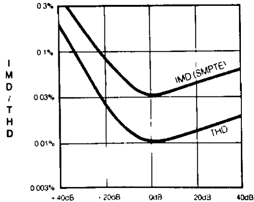
CURRENT GAIN/ATTENUATION (at 12dB Headroom 1kHz (BANDWIDTH 20kHz) ( 600\mu A_{pp} Constant Output Level) 0dB to +40dB ( 600\mu A_{pp} Constant Input Level) 0dB to -40dB)
