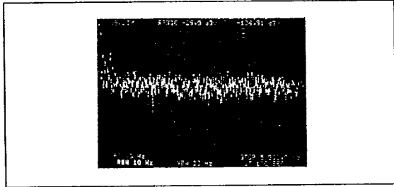
FIGURE 2: Spectrum Analyzer Display of Wideband Amplifier Noise Spectral Density. e_n \approx 1.7nV/\sqrt{Hz}
